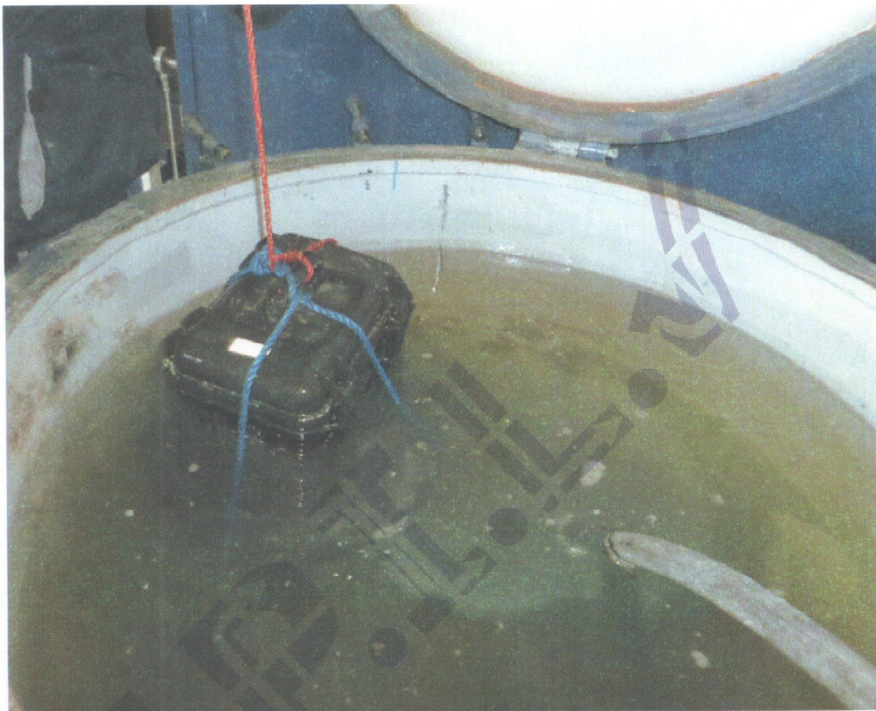
Figure 3: EUT under IPX7
