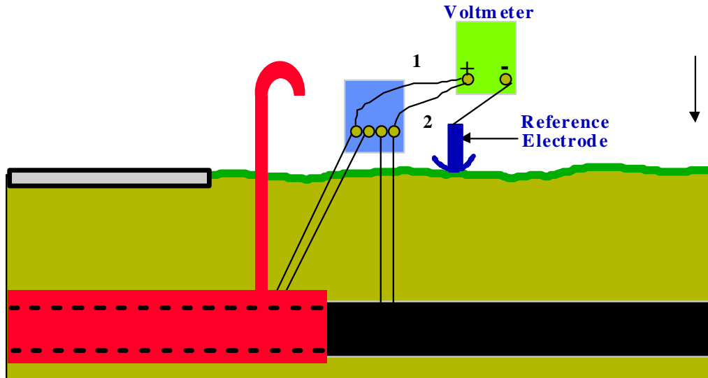
Figure 7-18 Testing for a Shorted Casing
