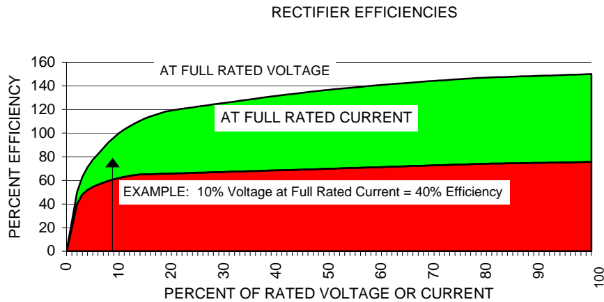
Figure 7-12. Rectifier Efficiency
